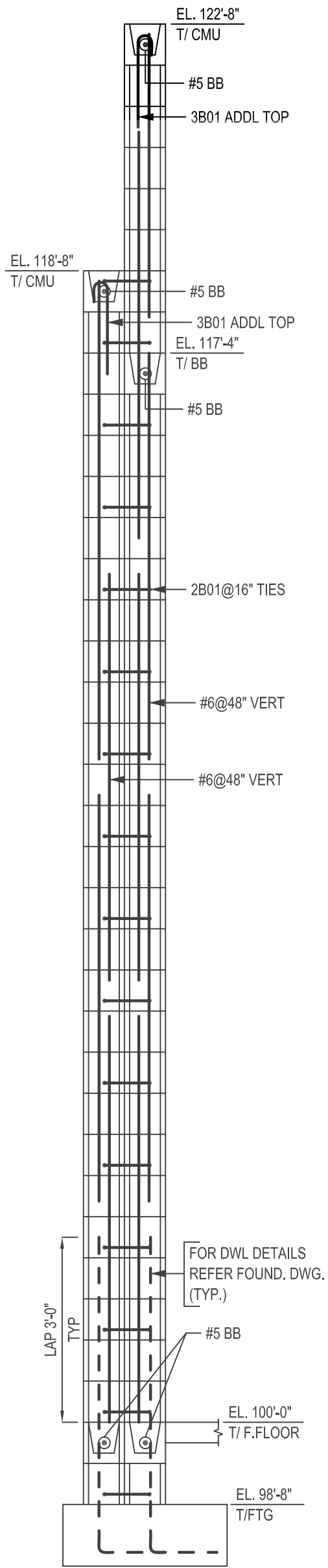
SECTION 2 SCALE: 1/2"=1'-0" SDR: 2/55 & 7/A3.3
