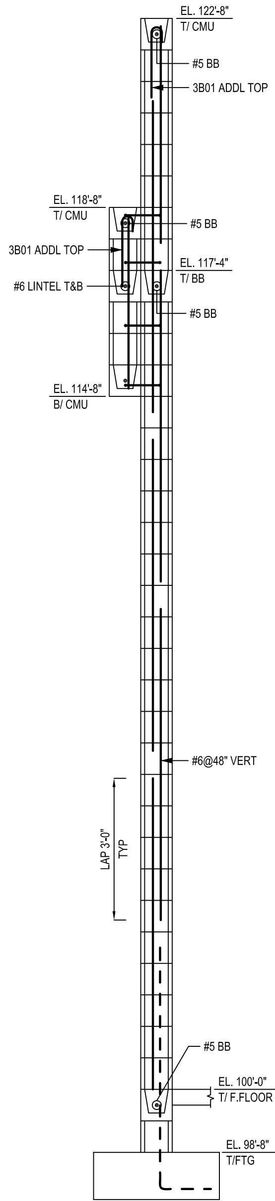
SECTION 1 SCALE: 1/2"=1'-0" SDR: 2/55 & 7/A3.3
